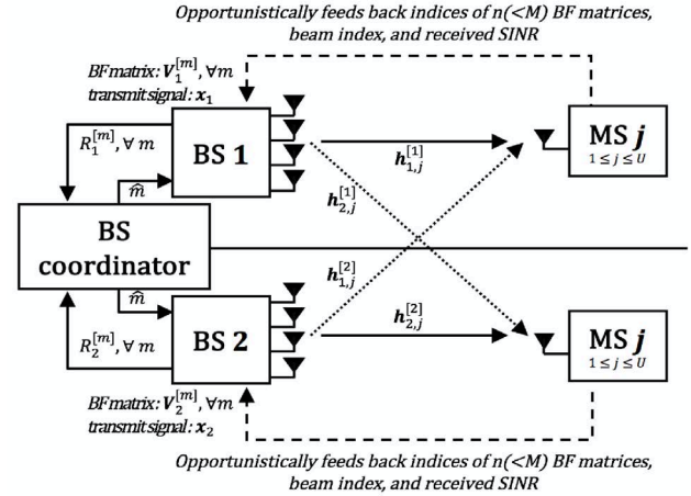
Fig. 1. System model of multi-cell downlink networks when K = 2 and N_t = 4
